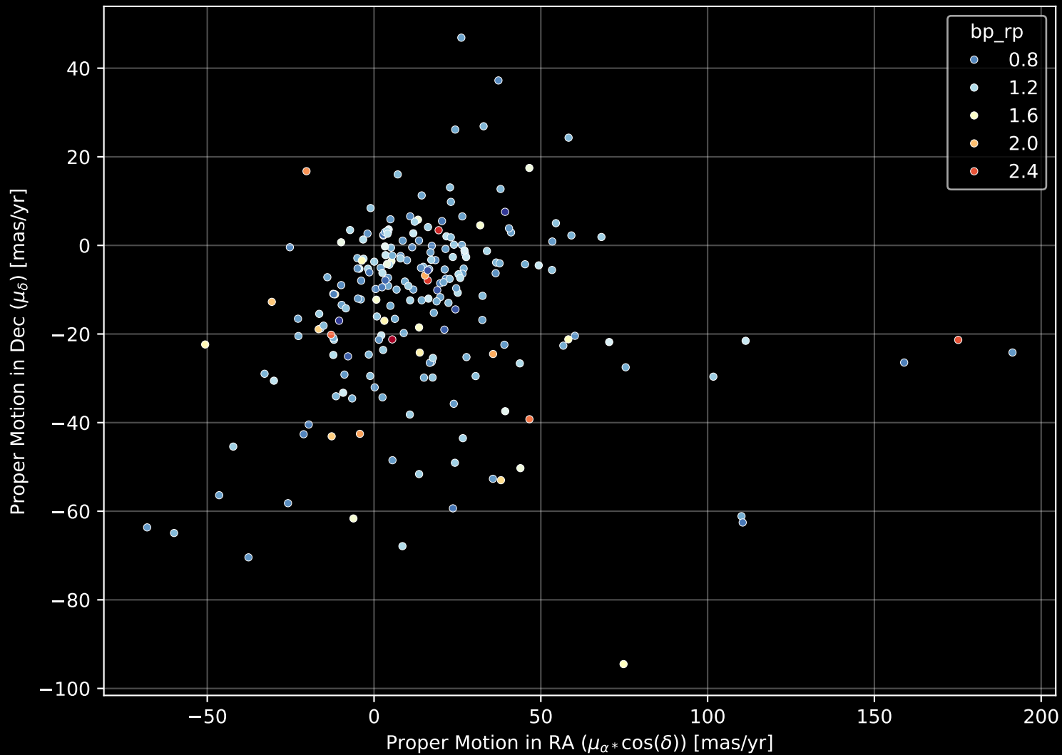
APOGEE DR17 Field: [134-51-O] Proper Motion Diagram (n= 216)
