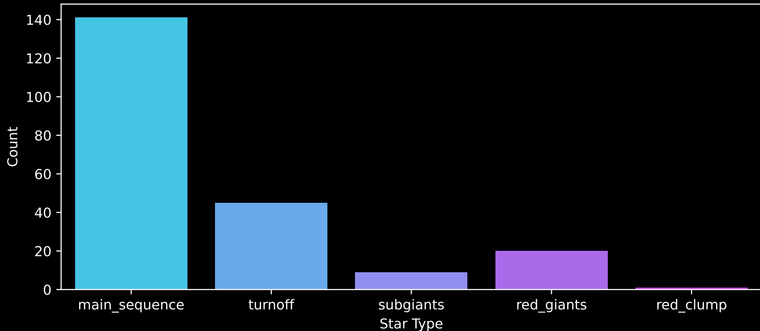
APOGEE DR17 Field: [134-51-O] Count plot of Star Type
