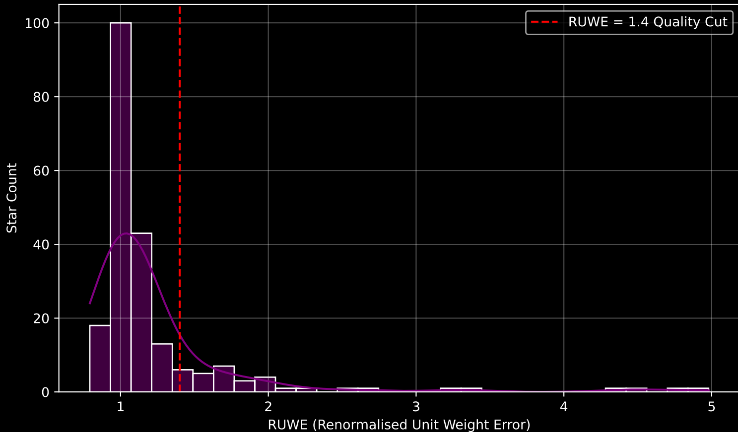
GAPOGEE DR17 Field [134-51-O] RUWE Distribution (n= 209)
