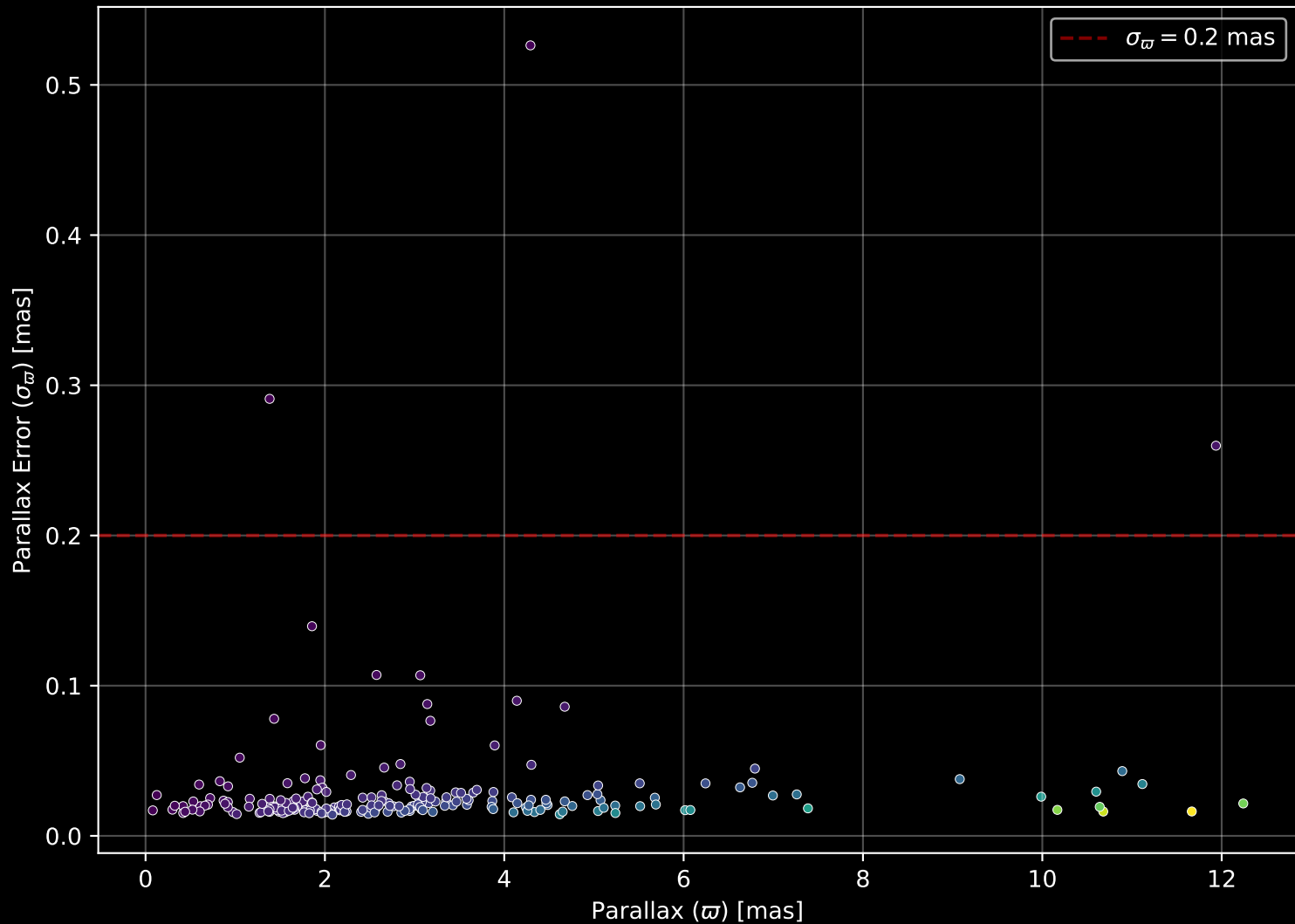
APOGEE DR17 Field: [134-51-O] Parallax Quality (n= 216)
