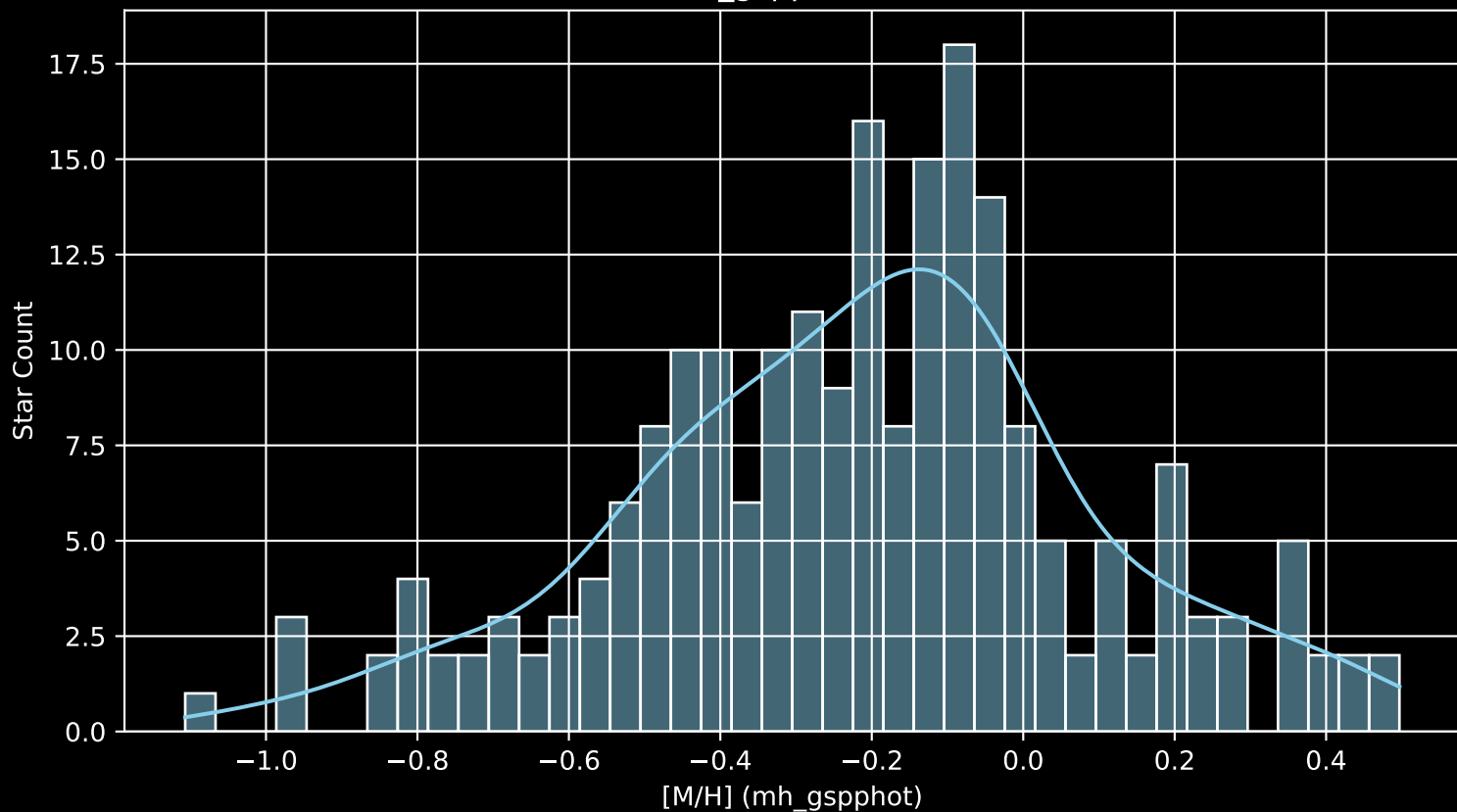
APOGEE DR17 Field: [134-51-O [M/H] (mh_gspphot) (n= 213)
