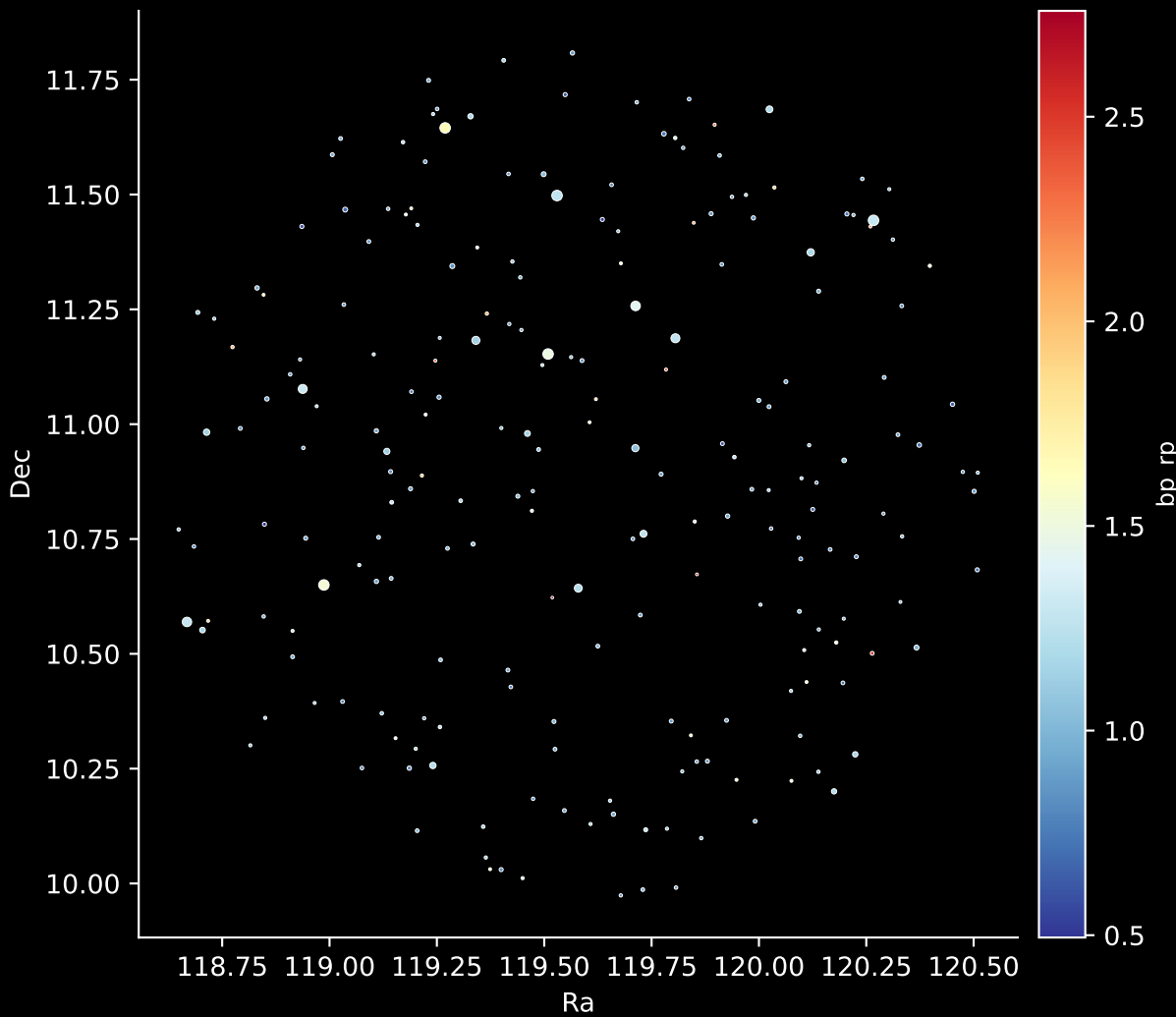
APOGEE DR17 Field: [134-51-O] Stars: 216
